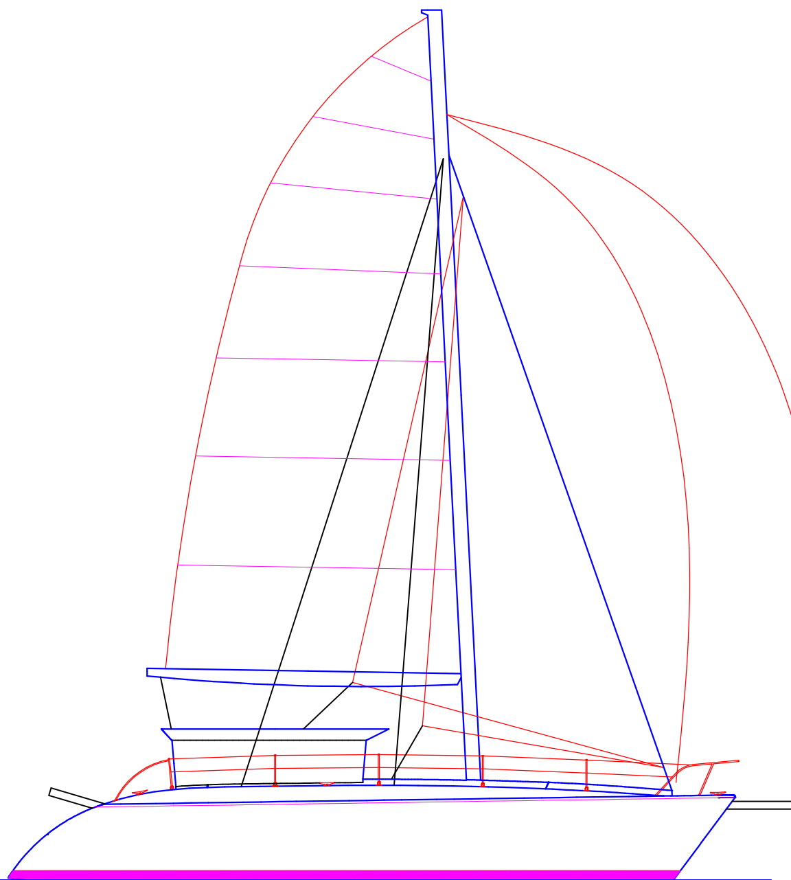
KSS46—pilot house Side View
