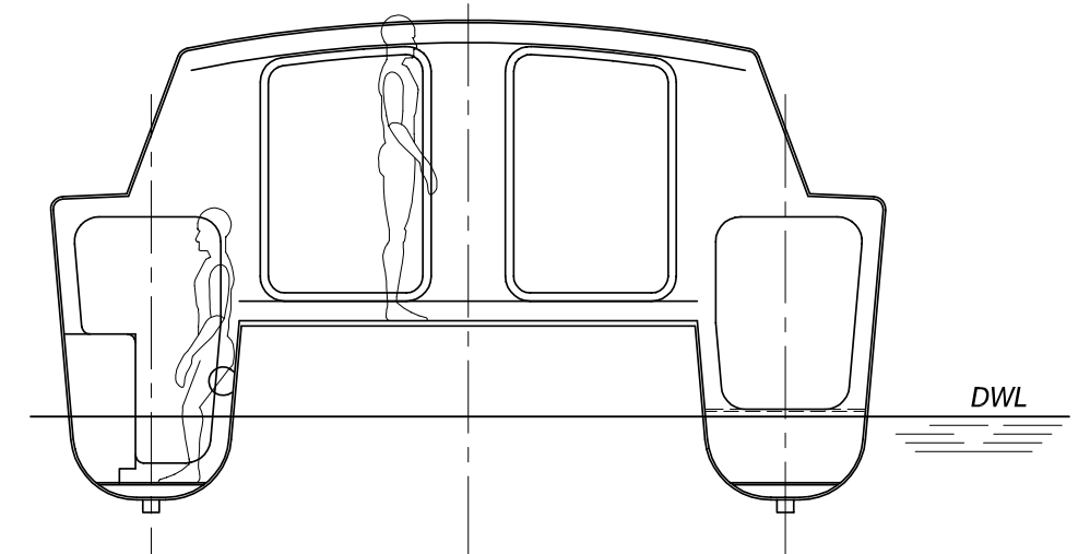
Section @ St. 5 looking aft
