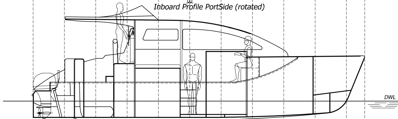
Inboard Profile StarBoardSide
