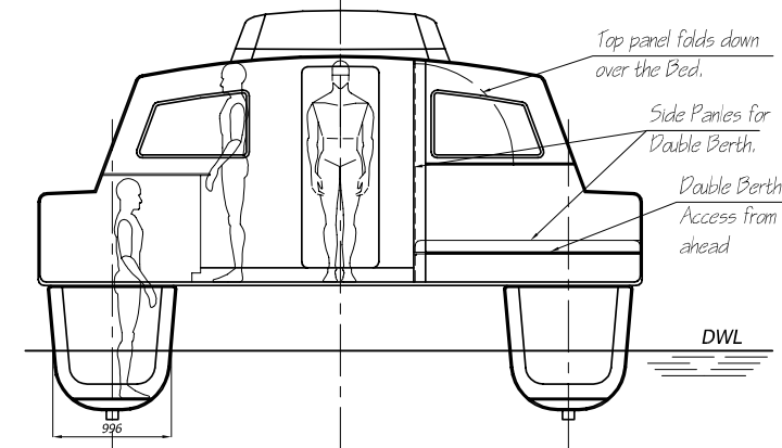
Section @ St. 5 looking aft
