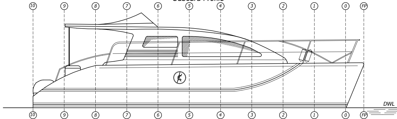
Inboard Profile PortSide (rotated)
